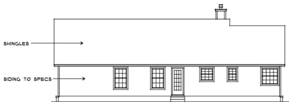
Rear Elevation
